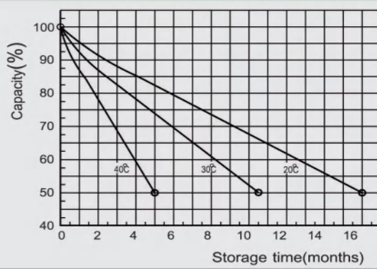
Self-discharge characteristics
