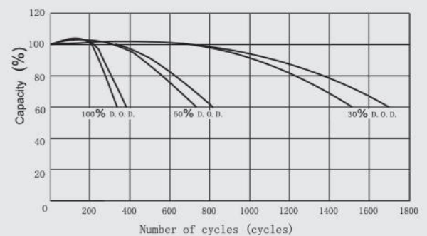
Cycle life on D.O.D (25°C)
