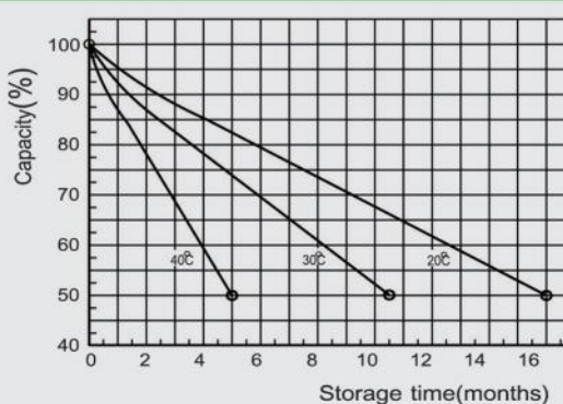
Self-discharge characteristics
