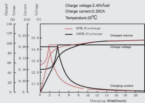
Charging characteristics
