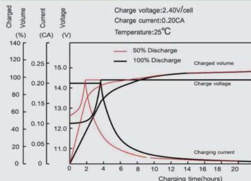
Charging characteristics
